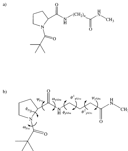
Scheme 1. a) Piv- 1 Pro-Xxx-NHMe, where Xxx = -\text{NH}-(\text{CH}_2)_n-\text{CO}- ( n = 1 , Gly; n = 2 , \beta -Gly; n = 3 , \gamma -Abu; n = 4 , \delta -Ava; n = 5 , \epsilon -Acp). b) Definition of the backbone torsional angles in Piv- 1 Pro- \gamma -Abu-NHMe.
